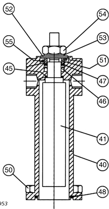
Stem Extension for 1/2" – 1-1/2" MK9020
